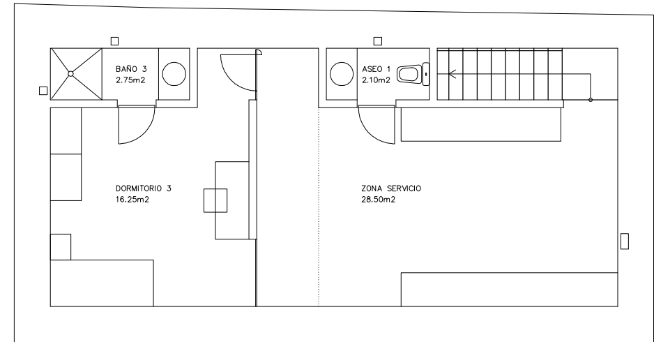
PLANTA SOTANO TOTAL SUP. UTIL 49.60 m² TOTAL SUP. CONST. 75.40 m²
